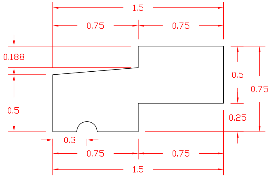
1-1/2" Water Table Drip Cap ATW-3029
