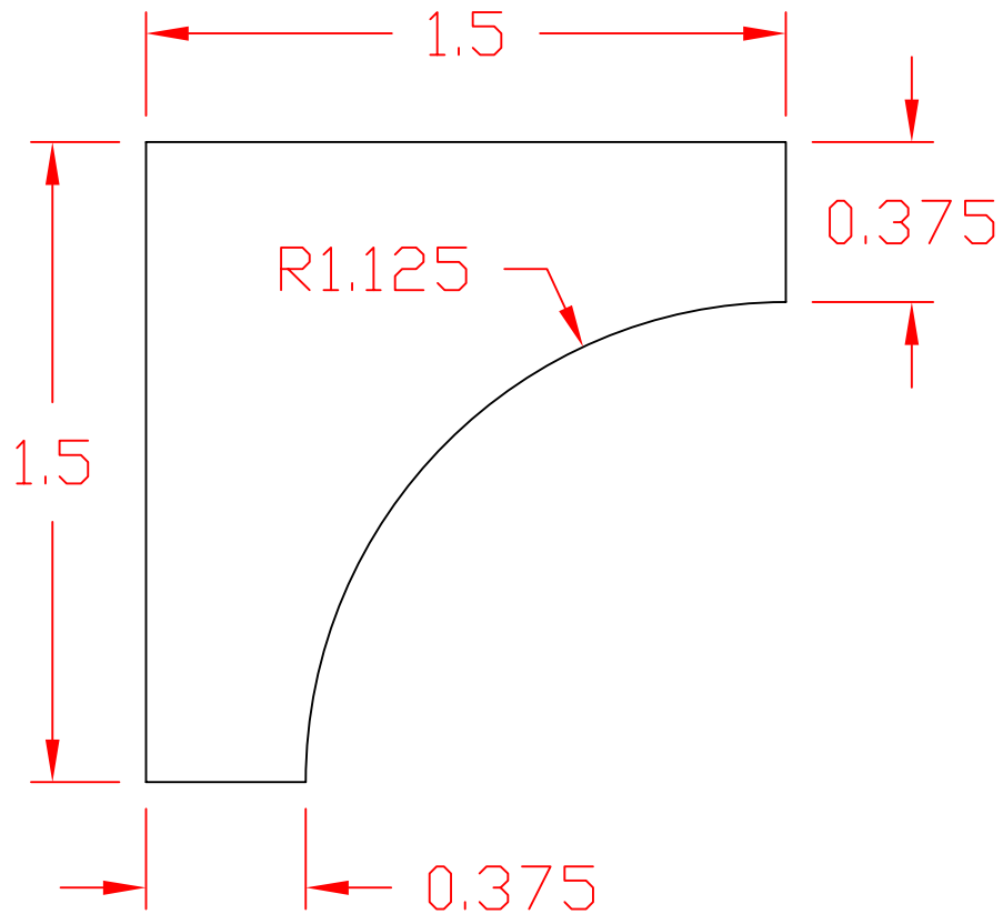
1-1/2" X 1-1/2" Cove (Scotia) Moulding ATW-3051
