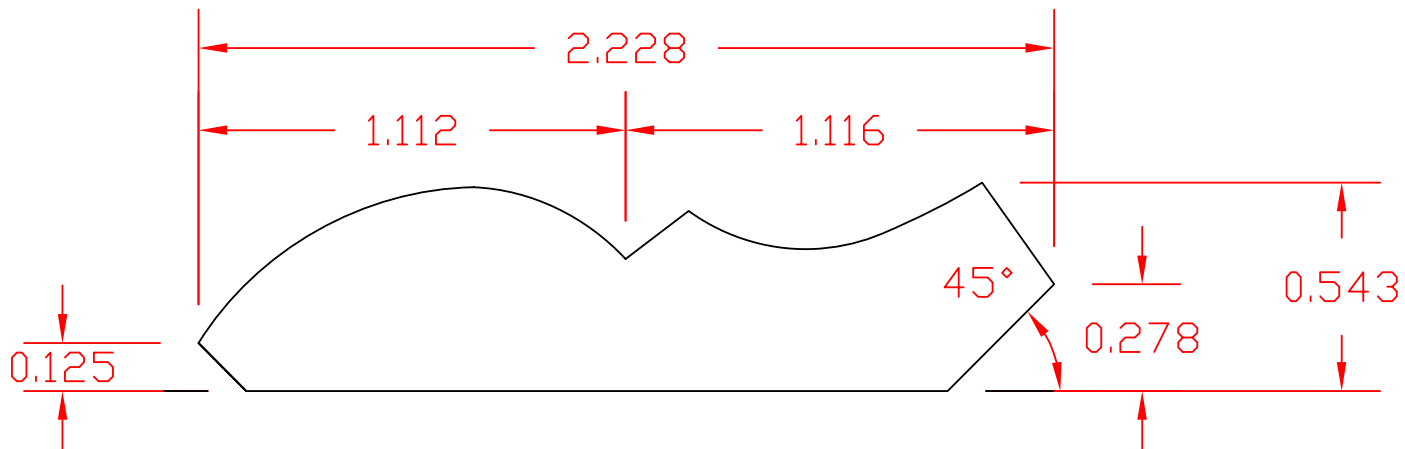
2-1/4" BED MOULDING ATW# 3075
