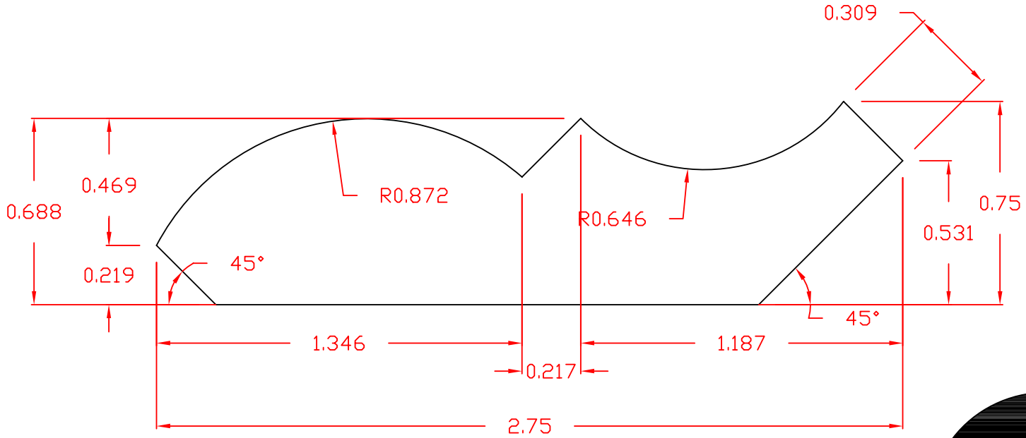
2-3/4" Bed Moulding ATW-3038
