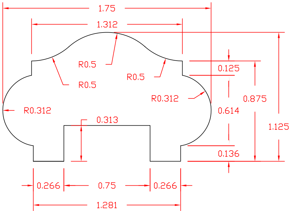
1-1/8" x 1-3/4" Nantucket Fence Cap with 3/4" dado ATW-3034
