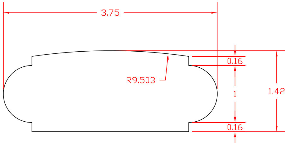
3-3/4" SMALL HANDRAIL ATW-3050
