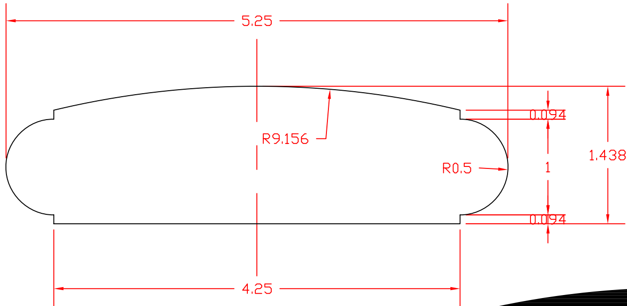
5-1/4" LARGE HANDRAIL ATW-3049
