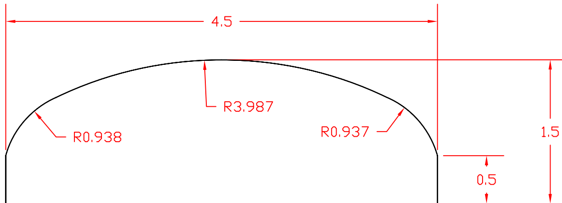
4-1/2" HAND RAIL ATW-3048
