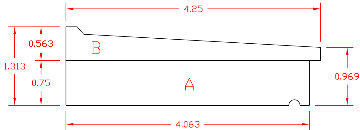
4-1/4" X 1-5/16" ANGLED DRIP CAP ATW-3085
