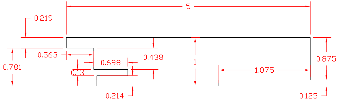
New Window Trim Kit W/ J-Channel
