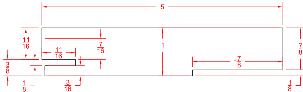
New Window Trim Kit ATW-3046
