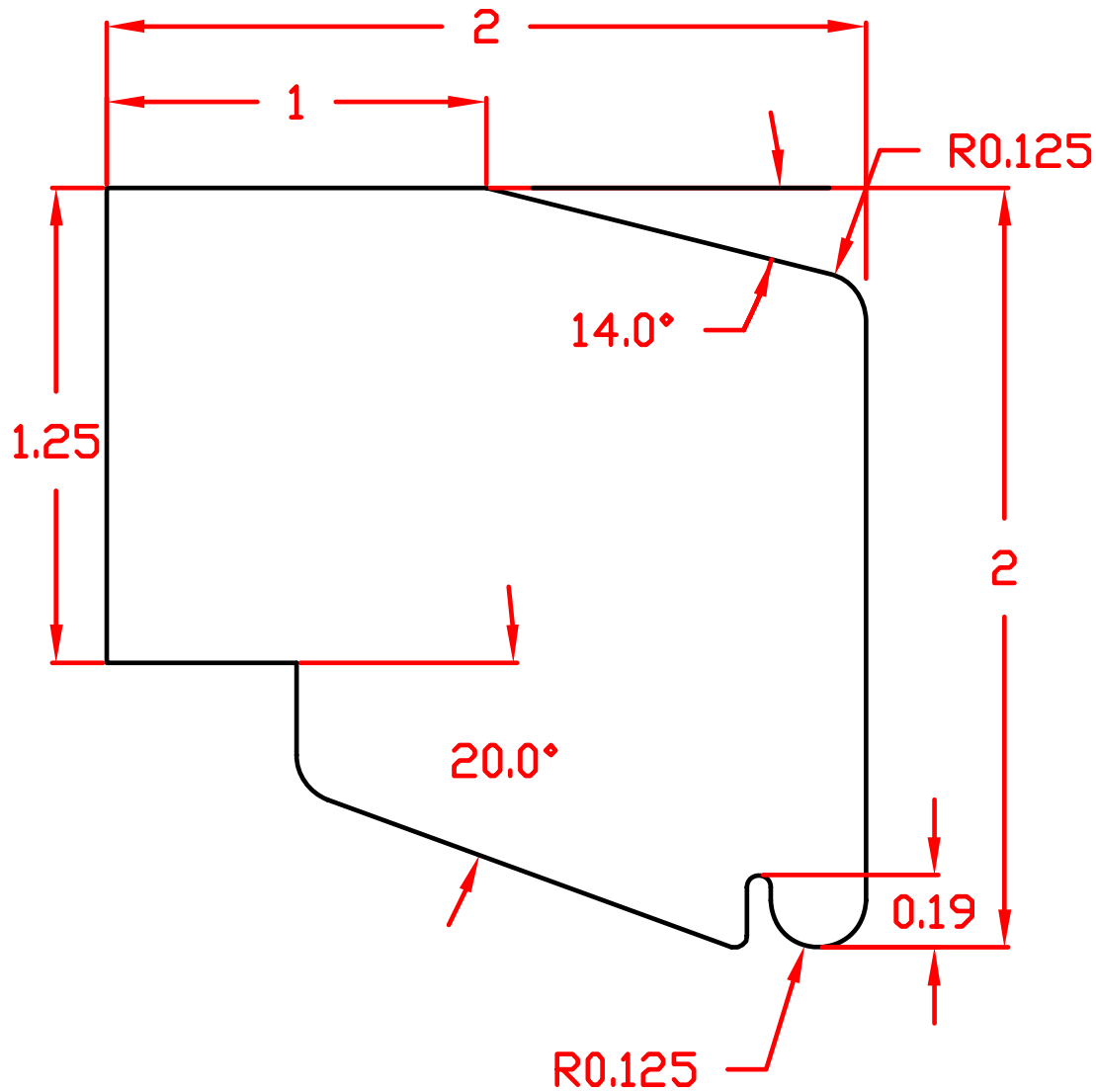
2" ATW STANDARD SILL ATW-3033
