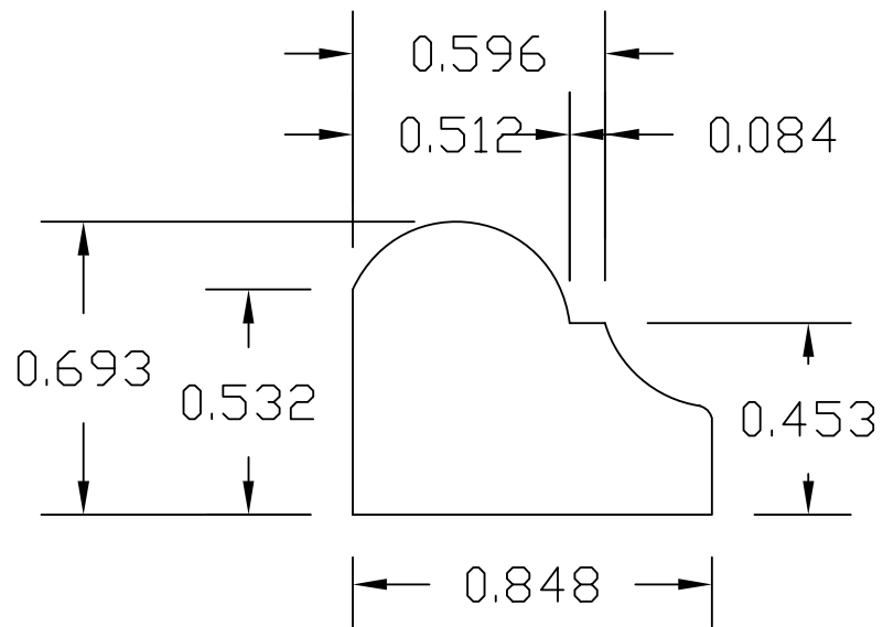
1/2" ROUND 1/4 COVE MOULDING ATW-3068
