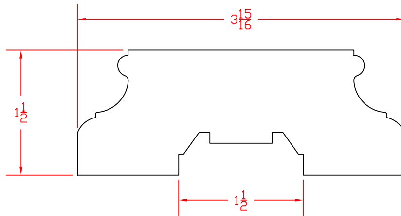
3-15/16" STANDARD DECKRAIL ATW-3086
