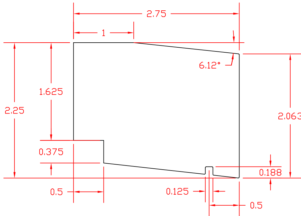
2-1/4" ATW HISTORICAL SILL ATW-3035
