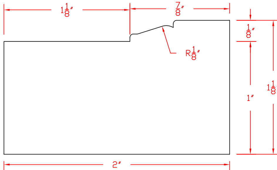
2" BBRICK MOULD (908 CASING) ATW-3032
